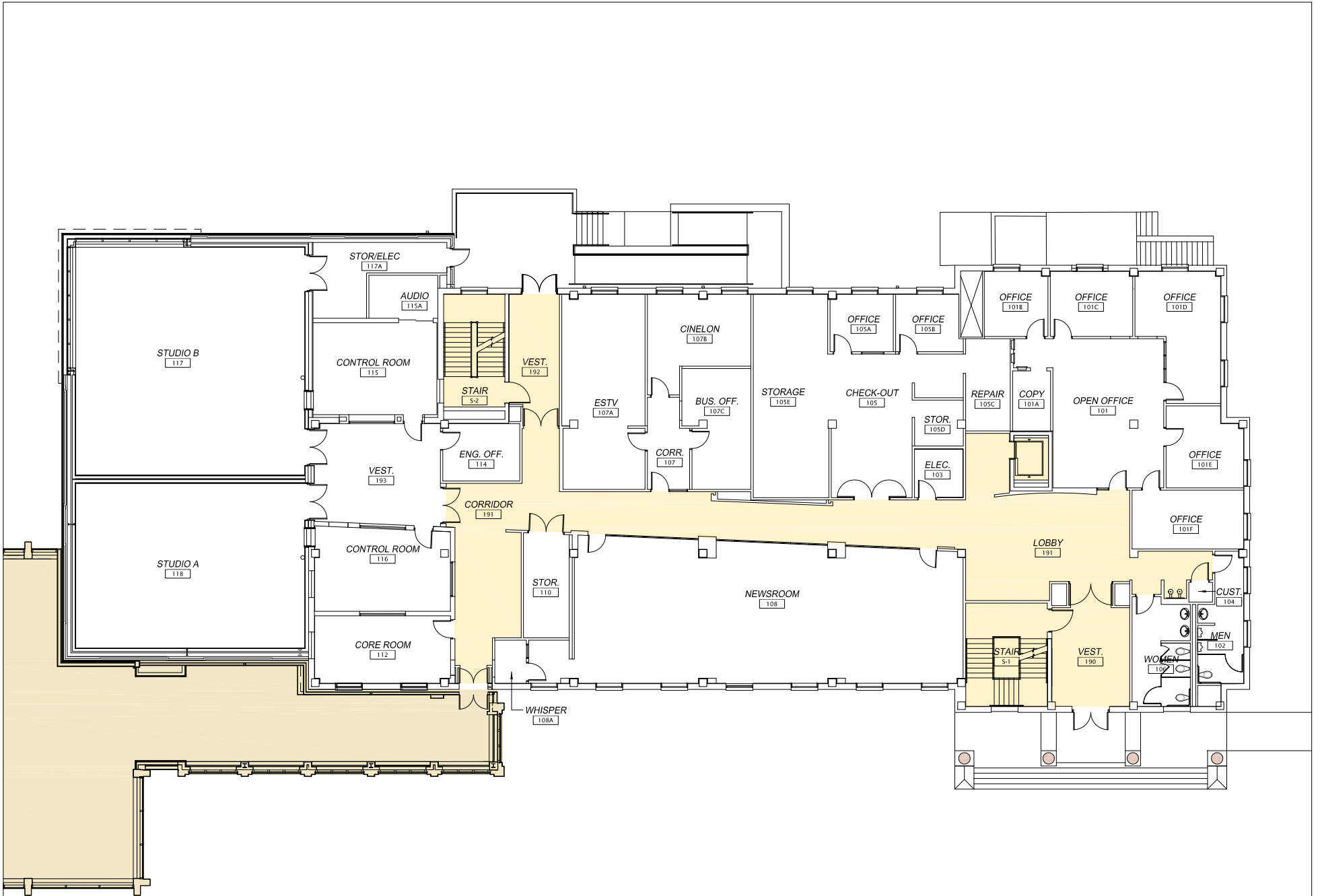
McEwen Hall First Level Plan
